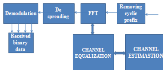
Figure 2. Receiver architecture
