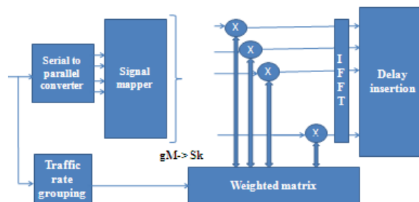
Figure 1. Transmitter architecture
