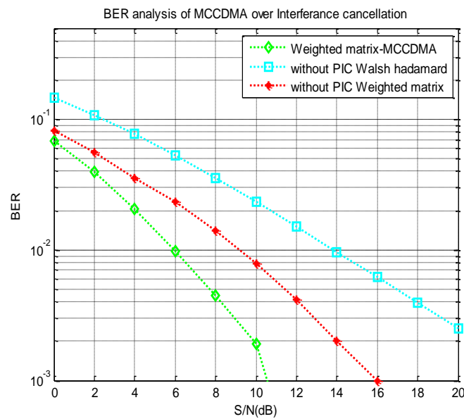
Figure 4. BER reduction with interference cancellation
