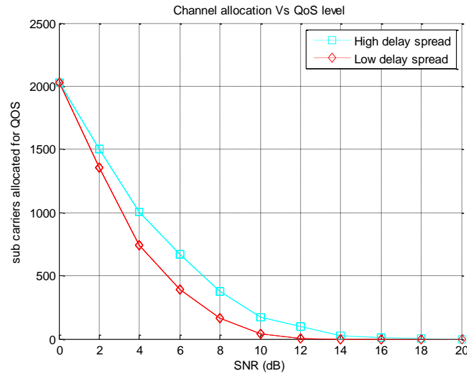
Figure 5. Qos driven carrier mapping analyzes
